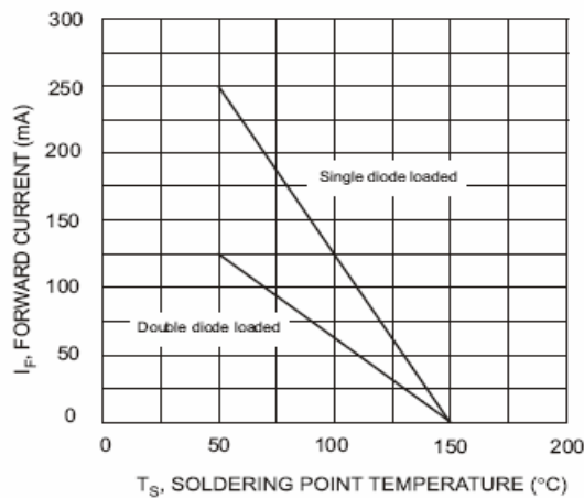
Fig. 1 Current Derating Curve
