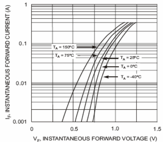
Fig. 2 Forward Characteristics
